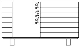
CGW02 L 150 x P 45 x H 85 cm
